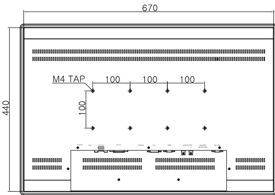
REAR VIEW
