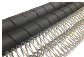
PLASTIC / SPRING GUARD SIZE : 1/4"~2" PLASTIC MATERIAL : HDPE SPRING MATERIAL : SUS 204, CARBON STEEL
