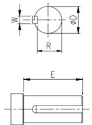
SHAFT EXTENSION
